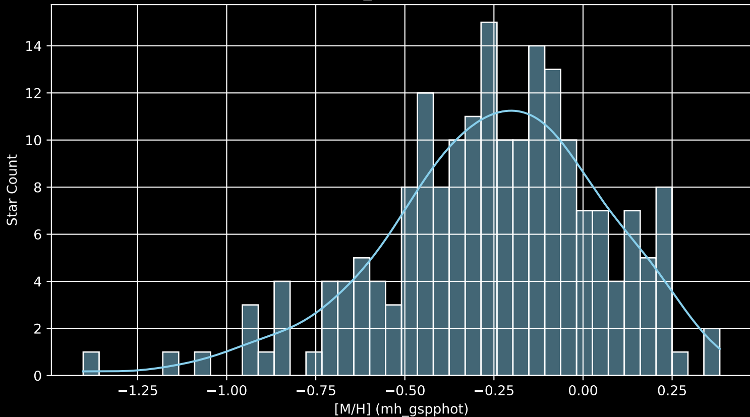
APOGEE DR17 Field: [K2_C5_210+34_btx [M/H] (mh_gspphot) (n= 194)
