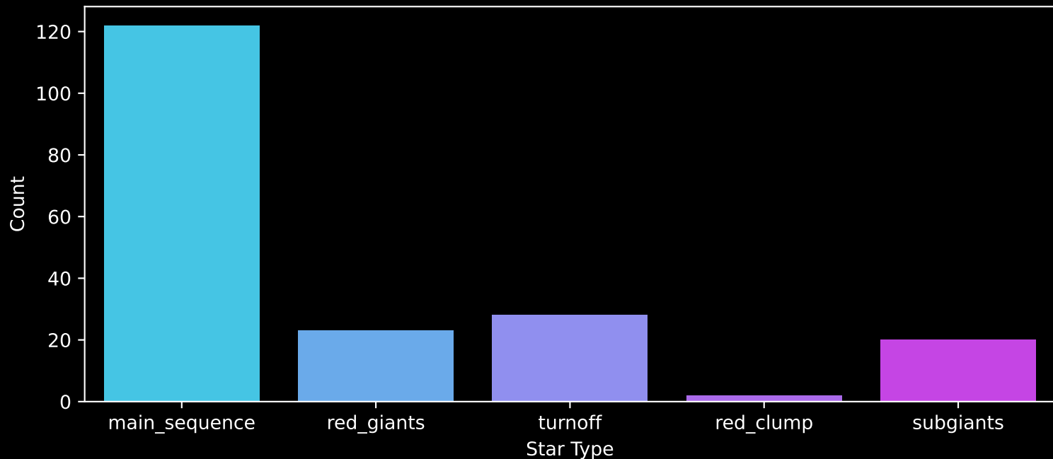
APOGEE DR17 Field: [K2_C5_210+34_btx] Count plot of Star Type
