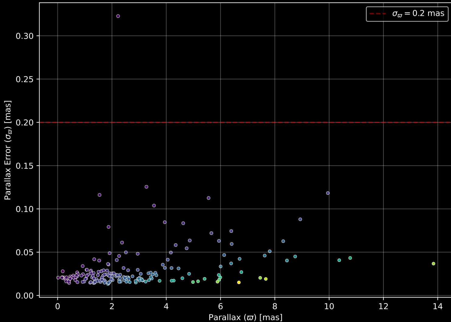
APOGEE DR17 Field: [K2_C5_210+34_btx] Parallax Quality (n= 195)
