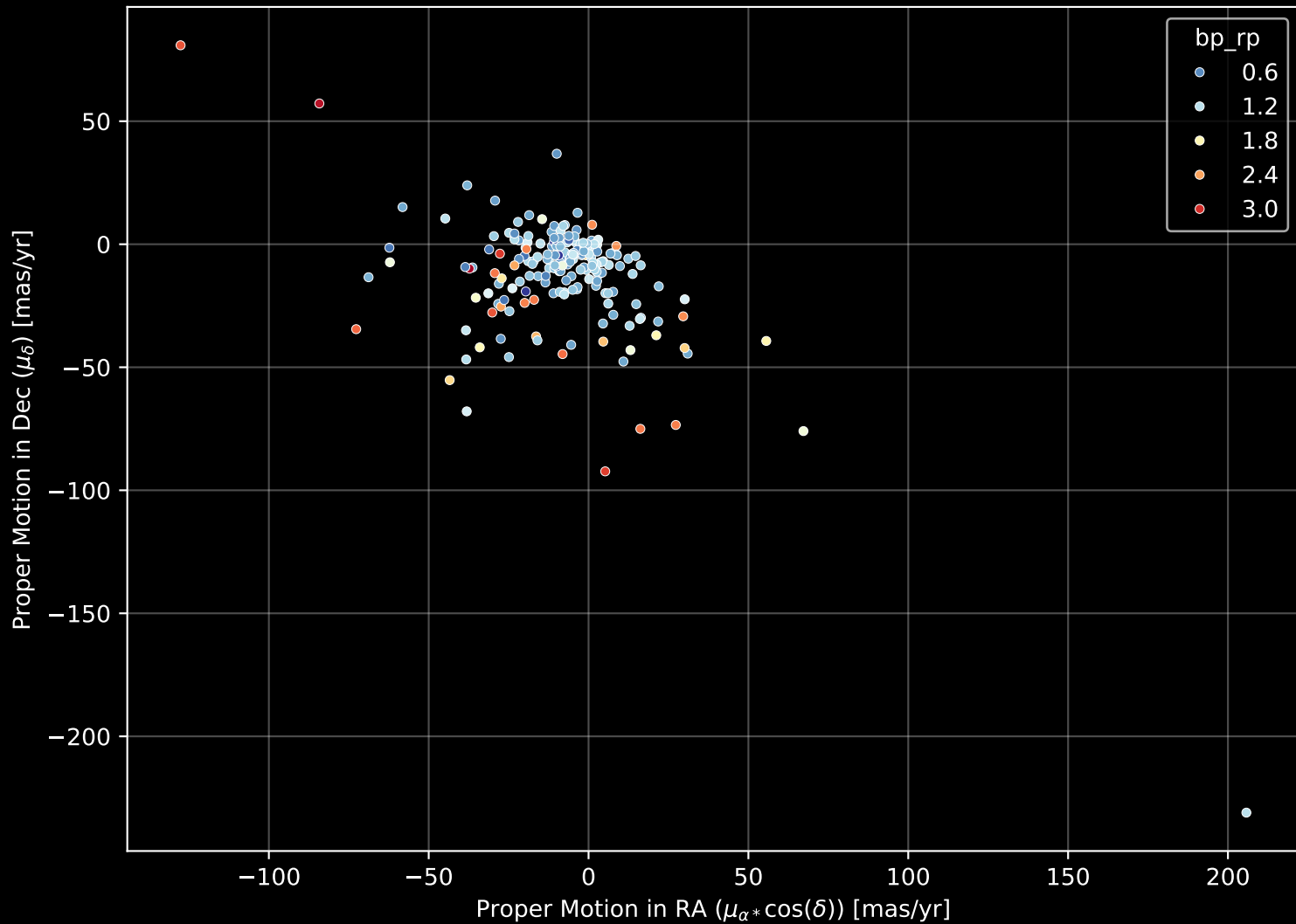
APOGEE DR17 Field: [K2_C5_210+34_btx] Proper Motion Diagram (n= 195)
