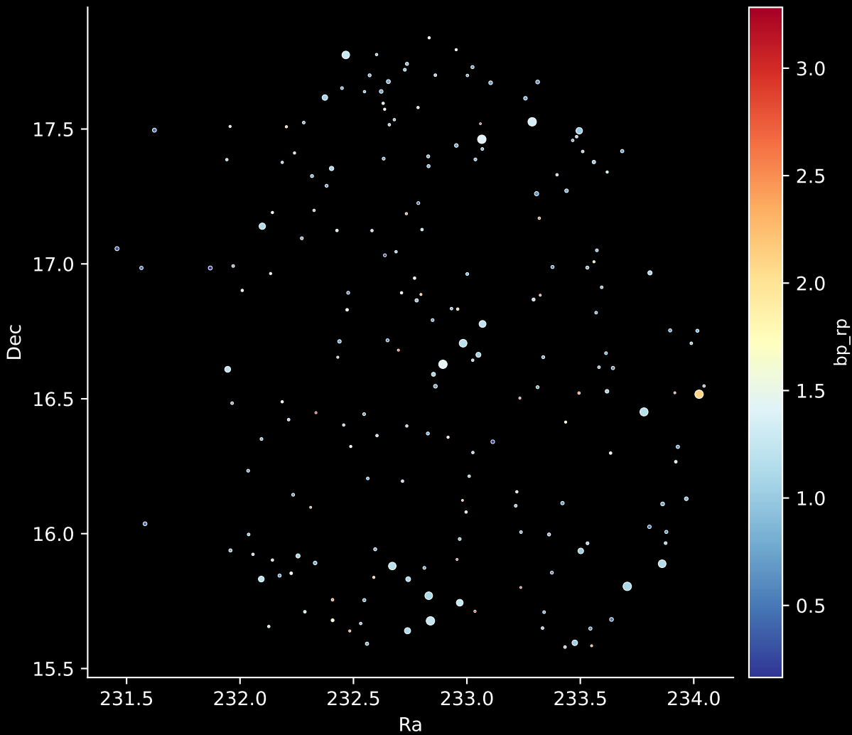
APOGEE DR17 Field: [K2_C5_210+34_btx] Stars: 195
