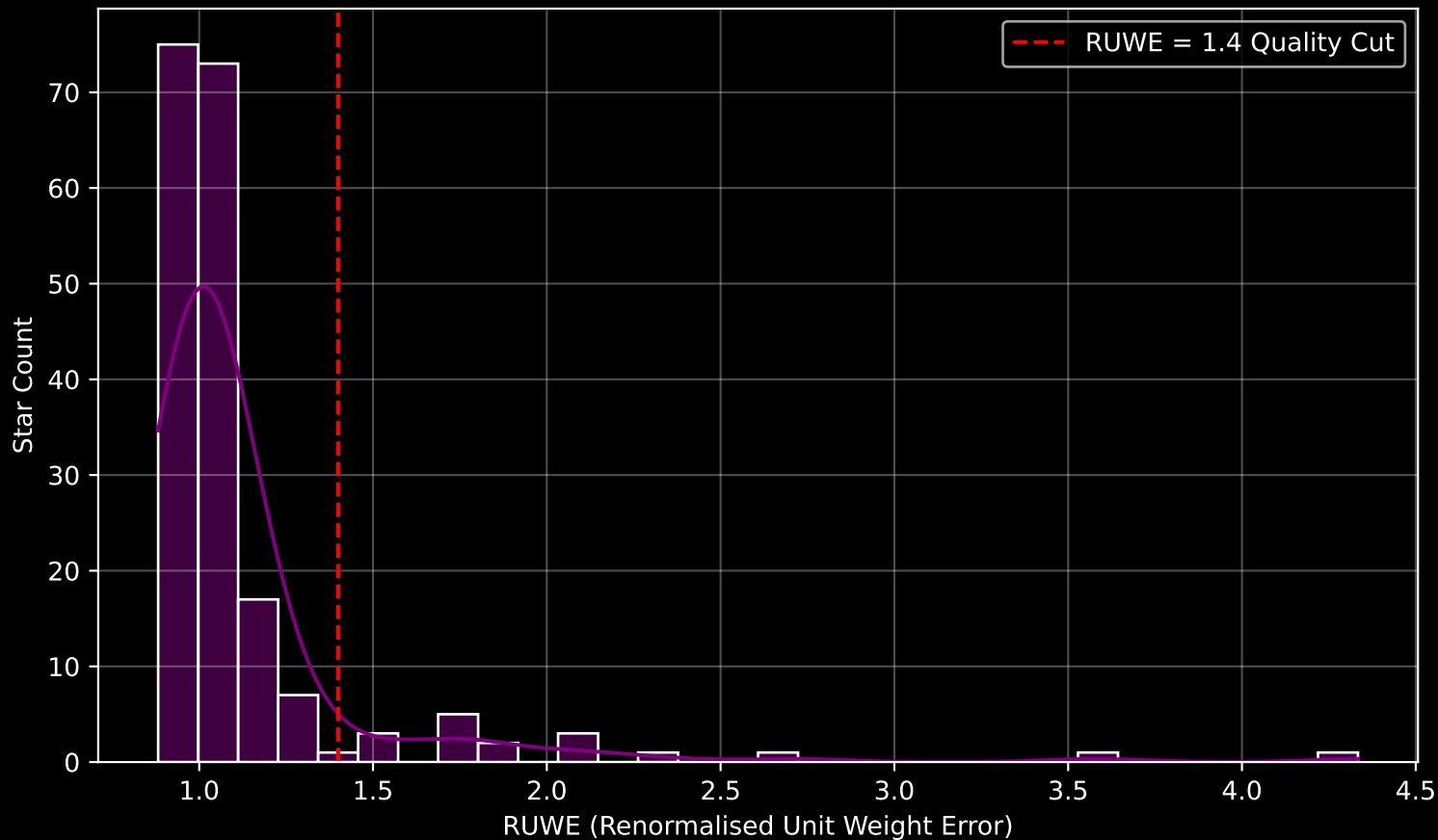
GAPOGEE DR17 Field [K2_C5_210+34_btx] RUWE Distribution (n= 190)
