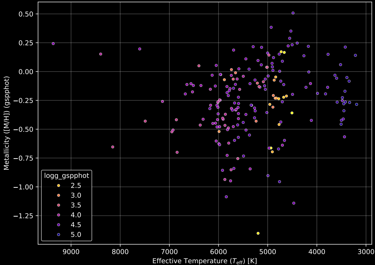
APOGEE DR17 Field: [K2_C5_210+34_btx] Stellar Population Parameters (n= 195)
